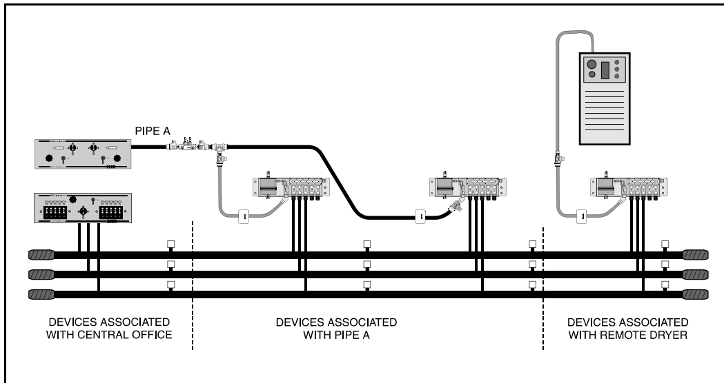
FIGURE 5-2: DEVICES ON OFFICE SIDE OF A REMOTE DRYER
