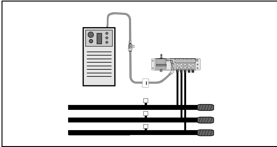
FIGURE 5-3: REMOTE DRYER AT THE END OF A CABLE RUN
