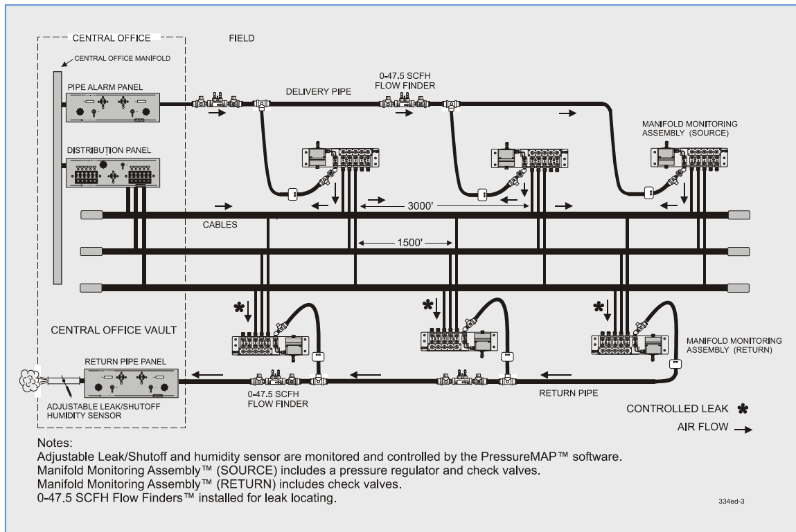
FIGURE A6-1: POSITIVE AIR FLOW SYSTEM
